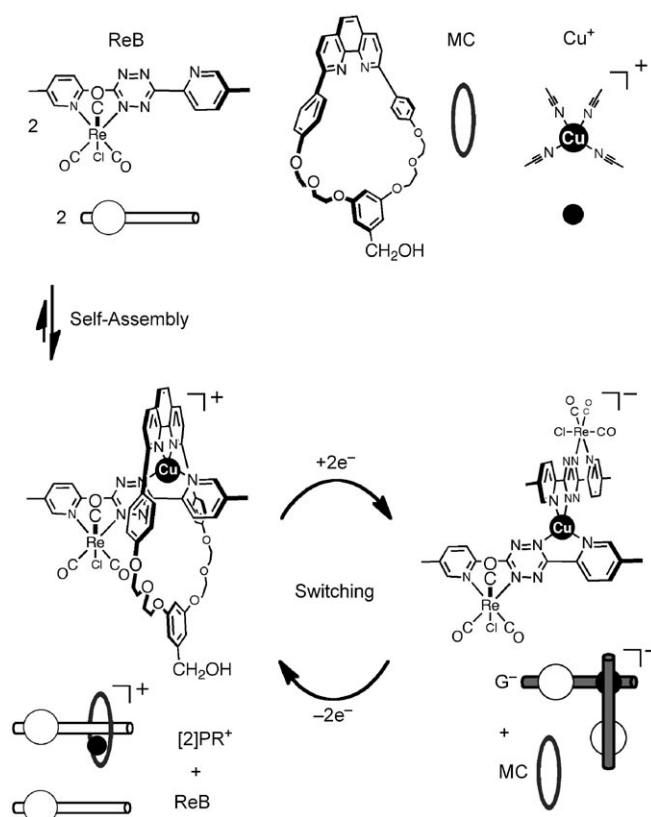
Scheme 1. A self-sorting mixture of two ligands (ReB and MC) around a \text{Cu}^{\text{I}} ion shows redox-driven interconversion between two distinct architectures: pseudorotaxane, [2]\text{PR}^+ , and grid-corner complex, \text{G}^- . (White and gray rods are neutral and reduced, respectively.)
